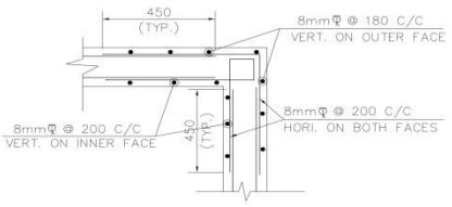
TYPICAL CORNER DETAILS IN PLAN
