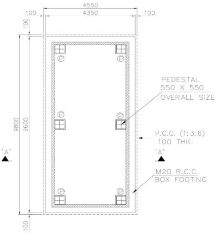
PLAN AT RAFT LEVEL
