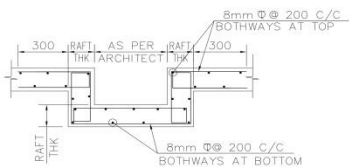
TYPICAL R/F DETAIL AT SUMP WELL (IF REQUIRED)
