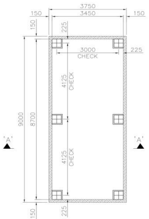
PLAN AT TOP LEVEL
